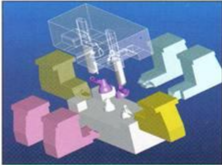
模具結構圖 Mould structure drawing →
